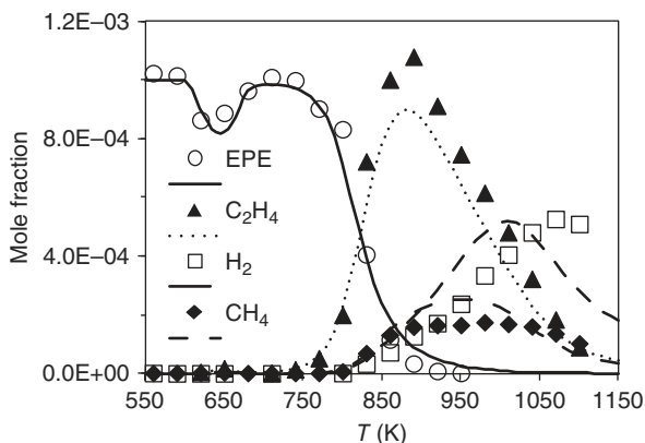
Figure 3.5 Experimental (symbols) and computed (lines) mole fraction profiles obtained from the oxidation of ethyl pentanoate in a JSR at \varphi=1 , p=10 atm, \tau=0.7 s (EPE, ethyl pentanoate).
