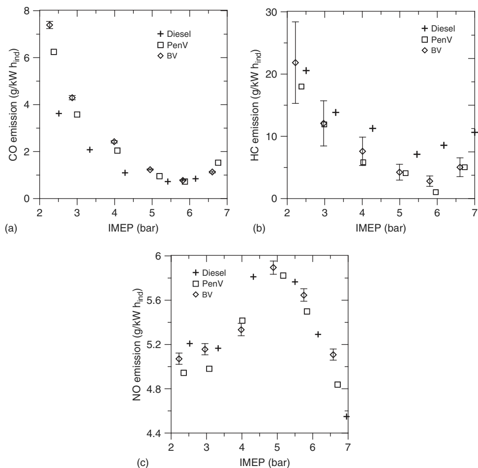
Figure 3.17 CO, unburnt HC, and NO emissions as a function of IMEP.
