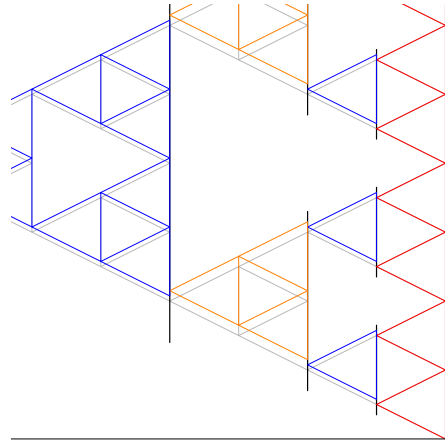
Fig. 3. When the head arrives in a computation window, it is here shifted upward, then upward again and downward in the third window. The state also changes then (red, later blue, orange and blue again). In light gray, another head whose position does not change.
