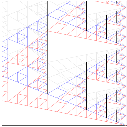
Fig. 2. Red and Blue (speeds 1 and 2) P-signals determine the positions of the lower points of the computation windows. In light gray, speed 5 and 6 P-signals that help determine the upper points.
