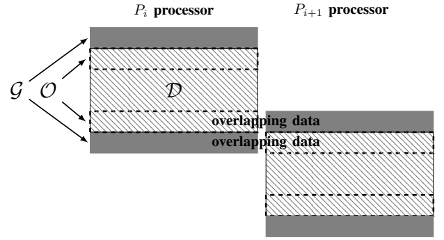
Fig. 3. Domain definitions for two processors with line bands
