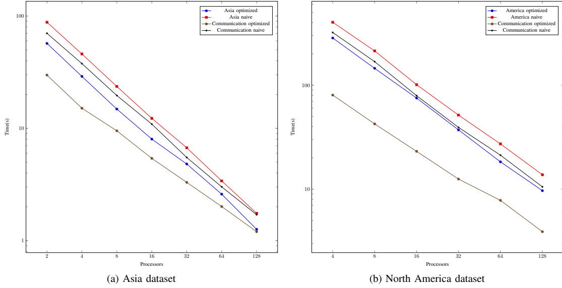
Fig. 5. Execution time of the labeling
