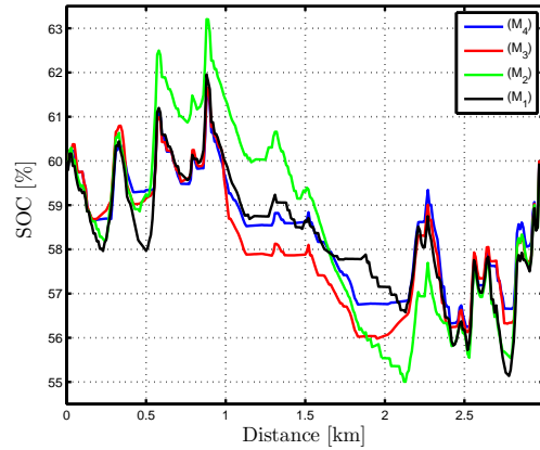
Figure 9: SOC [%] for LWLTC.
