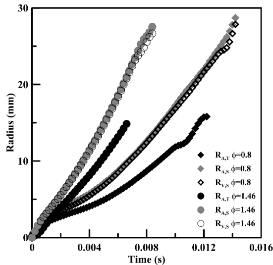
Figure 3. Example of different radii time evolution for lean and rich mixtures ( P=0.1 MPa, T=423\text{K} , u'=1.04 m/s).
