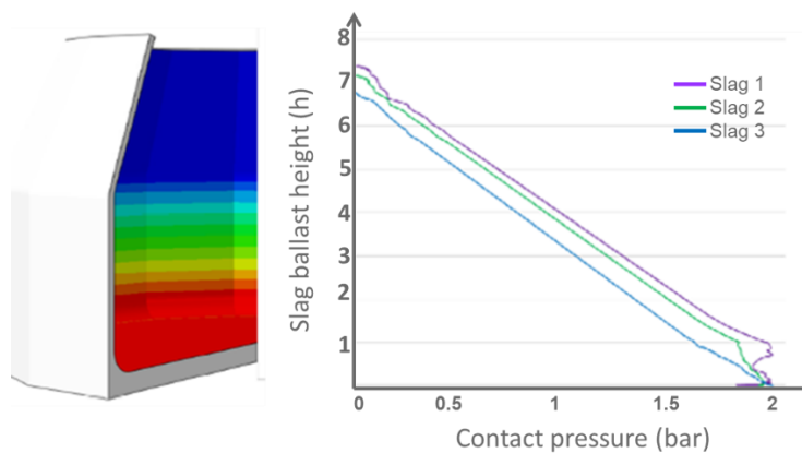
Figure 12: Contact pressure generated by slag expansion (5%) in actual GBS
