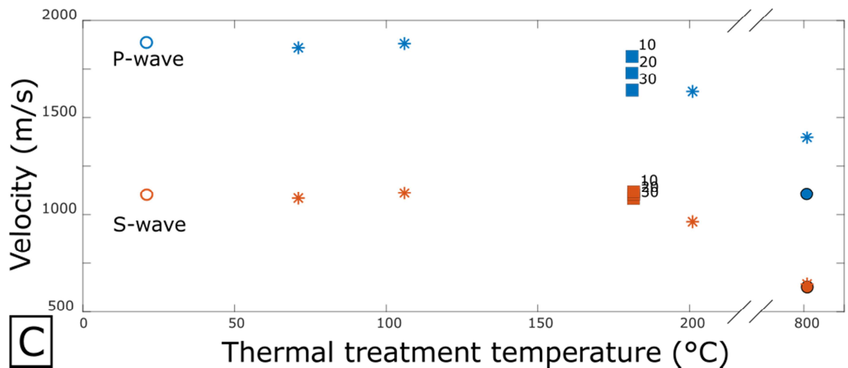
Figure 4. P- and S- wave velocities obtained a) for the siliceous concrete, b) for the calcareous concrete and c) for the Tuffeau. Blue dots are P-waves, orange dots are S-waves. The empty circle is the initial state, stars are the measurements obtained after thermal shocks, the squares are after the successive cycles and the filled circle is the measurement obtained after the high temperature treatment. For each point, the error bar is about \pm 50 m/s which is approximately the dot size.
