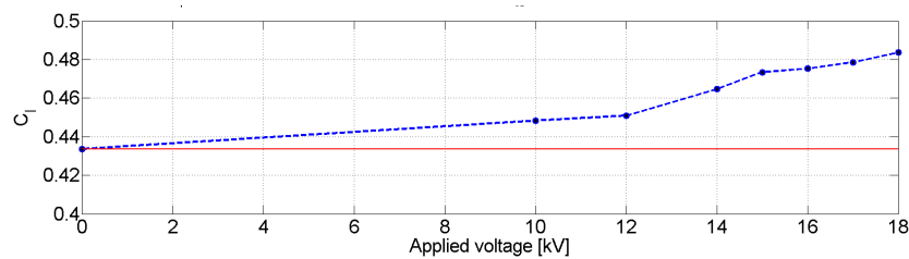
Figure 10. Lift coefficient as a function of the applied voltage (ACT1, U_\infty = 10m/s , \alpha = 0^\circ )
