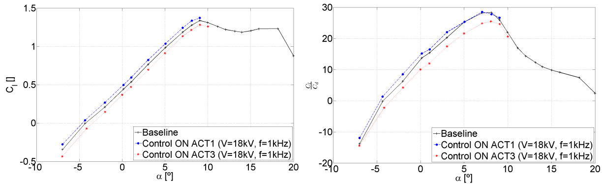
Figure 9. On the left, lift coefficient as a function of the angle of attack; on the right, lift to drag ratio as a function of the angle of attack ( U_\infty = 10m/s ( Re = 200000 ))
