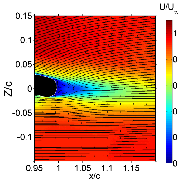
Figure 14. Non dimensional mean magnitude velocity field for ACT1 without actuation at \alpha = 0 and U_\infty = 10m/s
