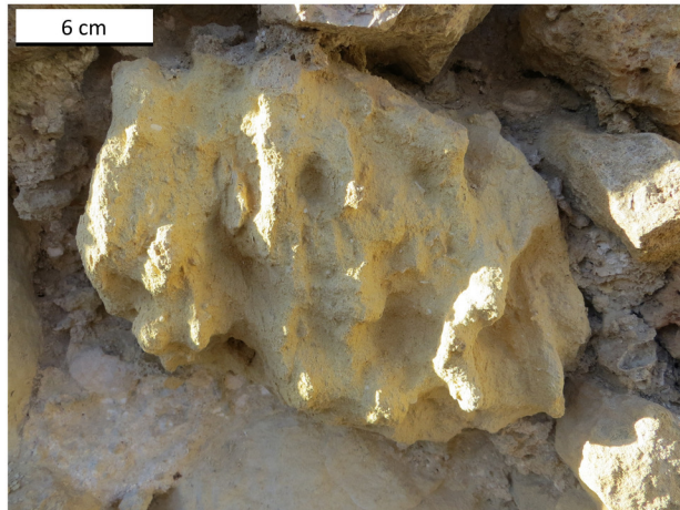
Alveolization
