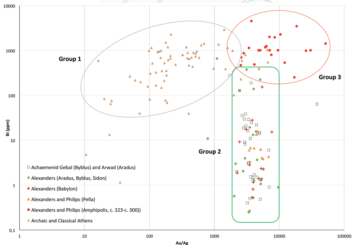
Fig. 10. Bismuth (Bi) content against gold to silver (Au/Ag) ratio for Greek silver coinages (6th-4th century BC), Philips and Alexanders (c. 330-300 BC), (logarithmic scale).
