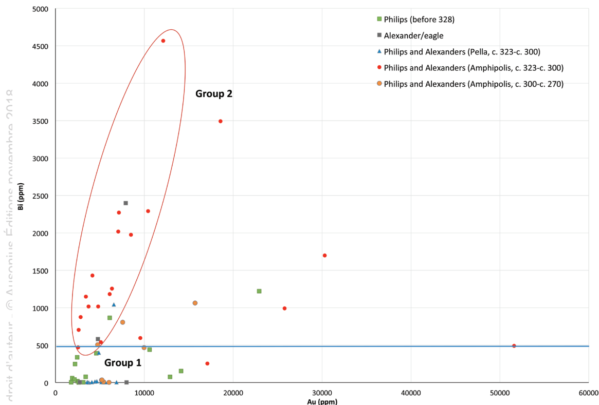
Fig. 7. Bismuth (Bi) content against gold to silver (Au/Ag) ratio for Macedonian coins ( c. 359- c. 270).
