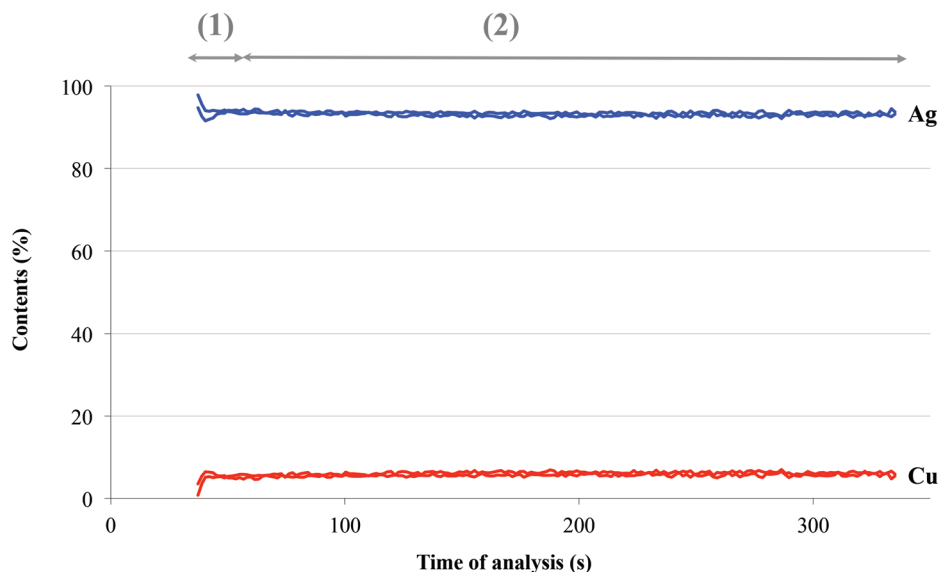
Fig. 2. Example of concentration depth profiles using LA-ICP-MS of silver and copper for the coin BnF MMA Delepierre 3006. (1) "Perturbed" surface layer; (2) "inner part" of the coin. Two micro-samplings were carried out. The laser was triggered at time 30 seconds.
