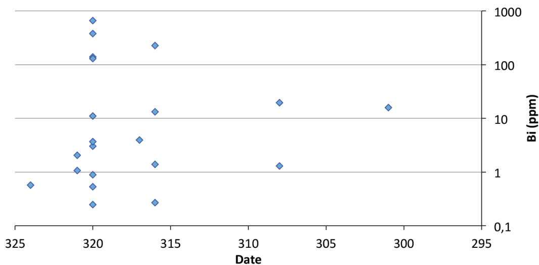
Fig. 5. Evolution of bismuth (Bi) content in Phoenician Alexanders.
