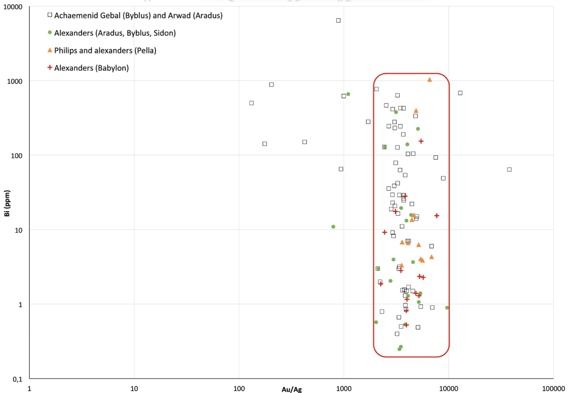
Fig. 9. Bismuth (Bi) content against gold to silver (Au/Ag) ratio for coins of Achaemenid Phoenicia, Babylon, and Pella.
