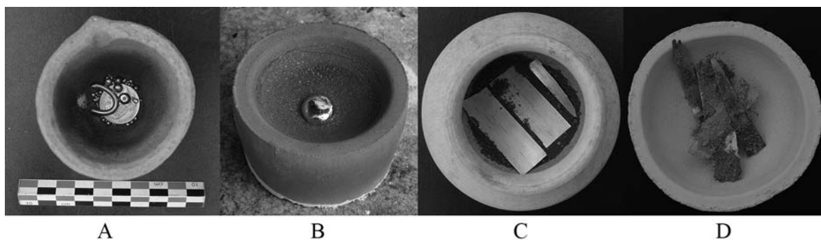
FIG. 1. The different steps of the archaeometallurgical experiments (from Blet-Lemarquand et al. 2014). From left to right, A: manufacture of the gold-silver-copper alloy; B: gold-silver alloy button obtained after cupellation; C: laminated foils made of gold-silver alloy in the cementation pot before cementation takes place; D: foils after cementation.
