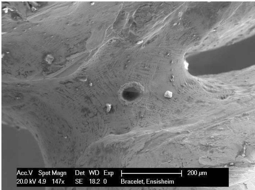
Figure 1. SEM images of laser ablation craters made on prehistoric gold artefacts using the two laser equipment available in the IRAMAT-CEB: (a) Nd:YAG; (b) ArF-excimer. © CNRS IRAMAT-CEB
