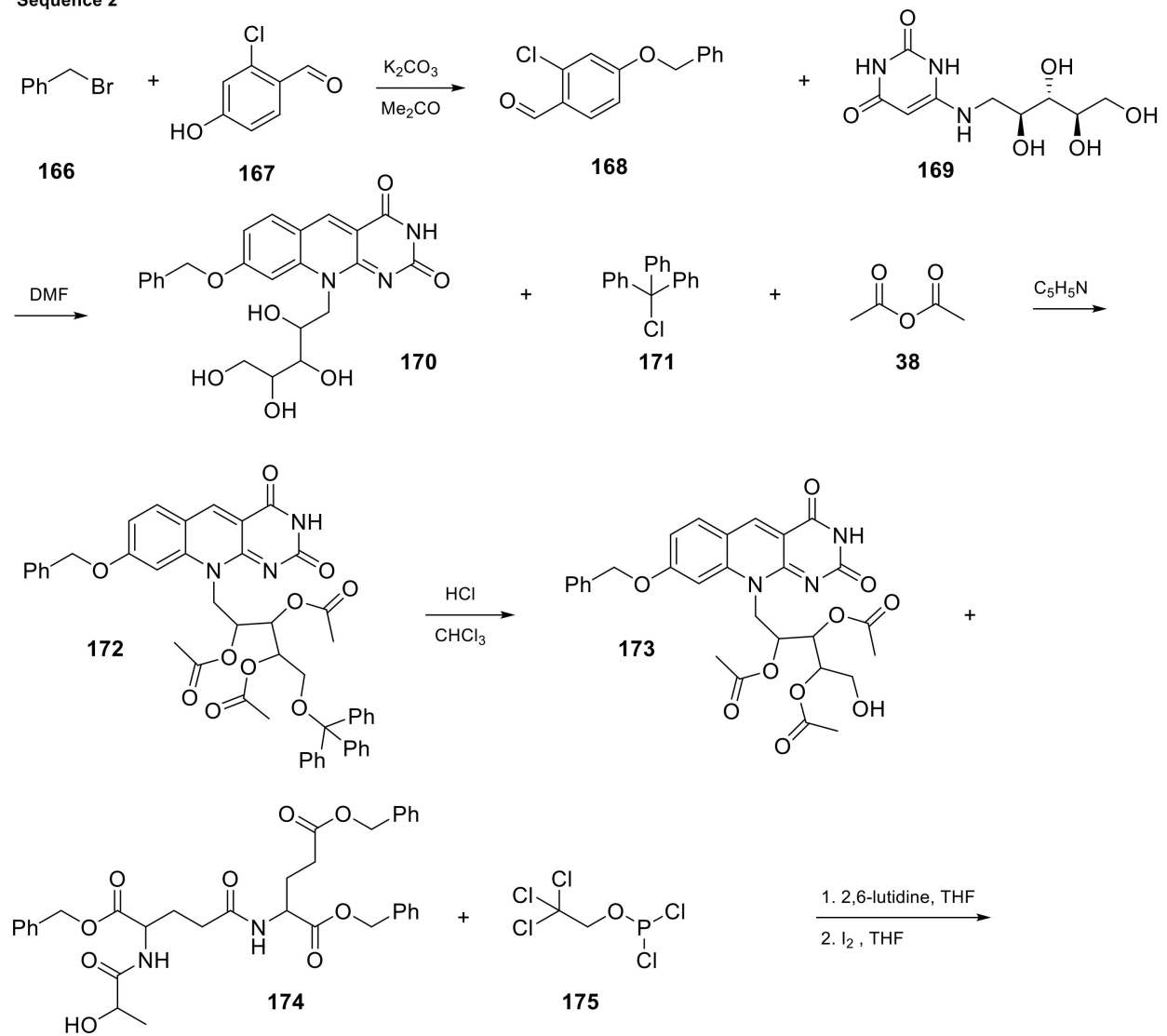
Scheme 18. Cont.
