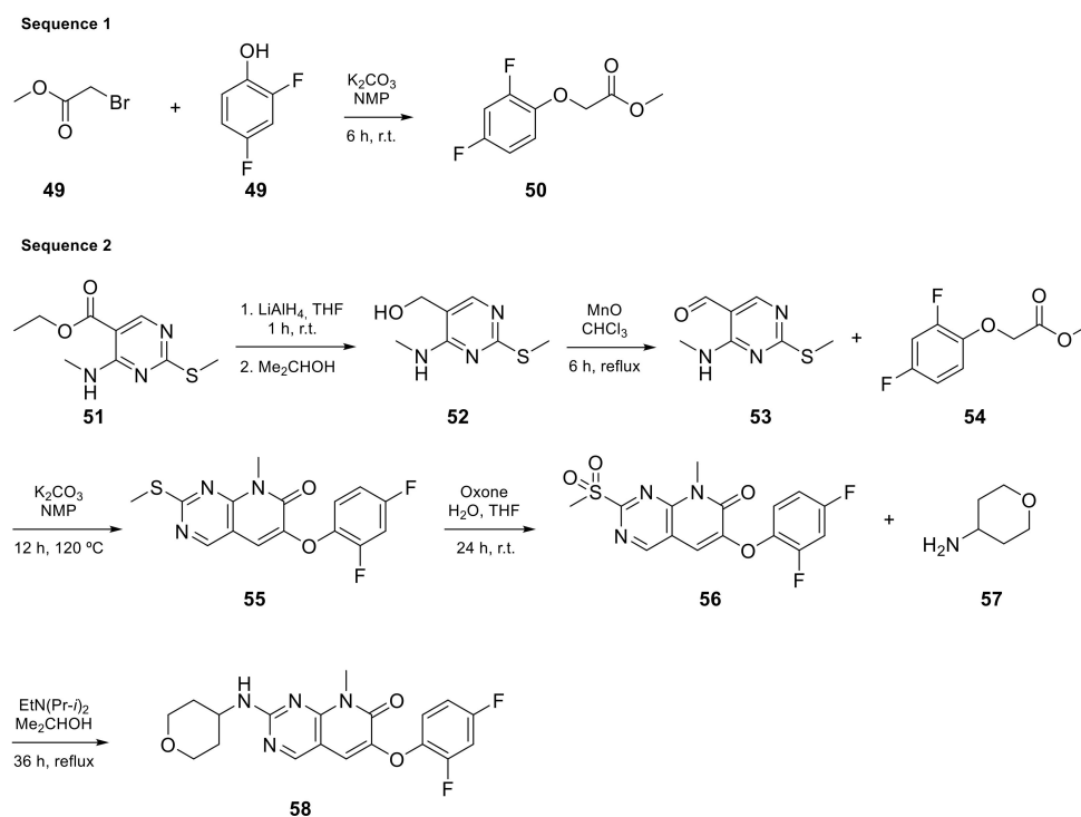
Scheme 8. Synthesis of 6-(2,4-difluorophenoxy)-8-methyl-2-[(oxan-4-yl)amino]-7H,8H-pyrido[2,3-d]pyrimidin-7-one ( 58 ) [29].
