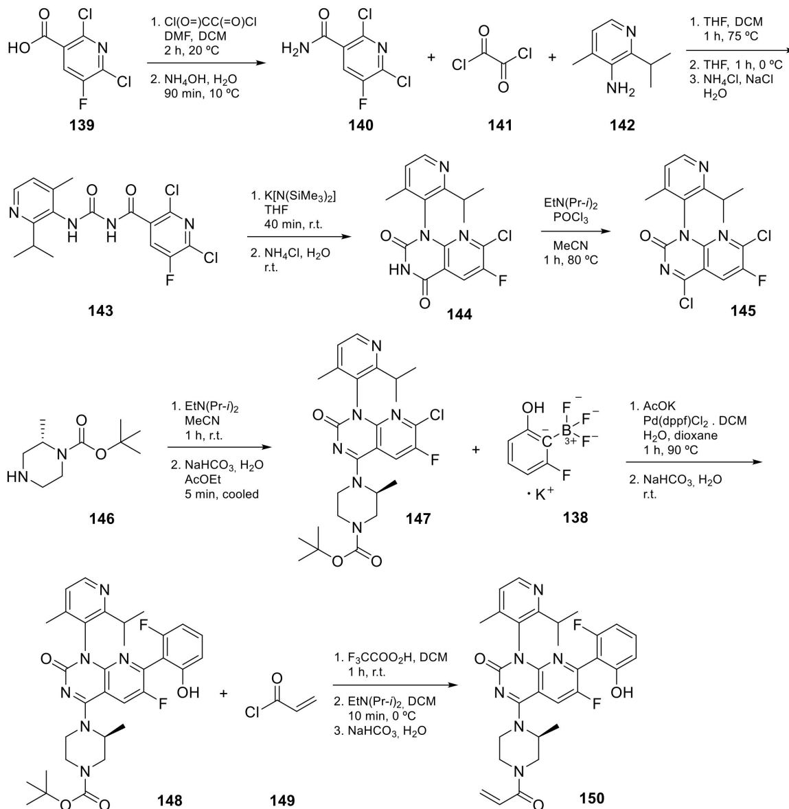
Scheme 15. 6-fluoro-7-(2-fluoro-6-hydroxyphenyl)-1-[4-methyl-2-(propan-2-yl)pyridin-3-yl]-4-[(2 S )-2-methyl-4-(prop-2-enyl)piperazin-1-yl]-1 H ,2 H -pyrido[2,3- d ]pyrimidin-2-one ( 150 ), AMG-510 [56].
