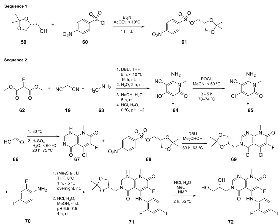
Scheme 9. Synthesis of 3-[(2R)-2,3-dihydroxypropyl]-6-fluoro-5-[(2-fluoro-4-iodophenyl)amino]-8-methyl-3H,4H,7H,8H-pyrido[2,3-d]pyrimidine-4,7-dione ( 72 ) [33].
