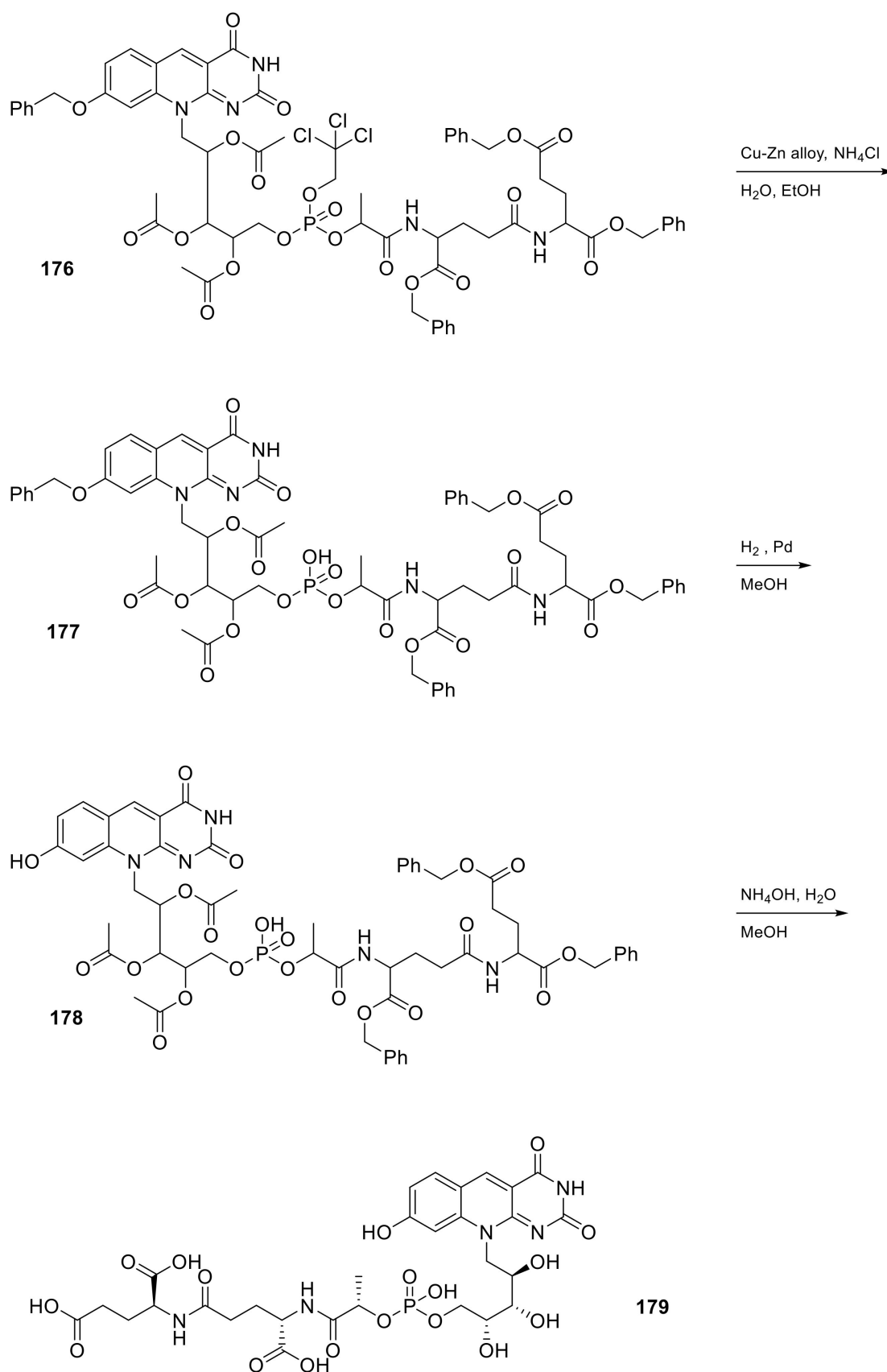
Scheme 18. (2S)-2-[(4S)-4-carboxy-4-[(2S)-2-[(hydroxy((1(2R,3S,4S)2,3,4-trihydroxy-5-(8-hydroxy-2,4-dioxo-2H,3H,4H,10H-pyrimido[4,5-b]quinolin-1-yl)pentyl]oxy))phosphoryl]oxy)propanamido]-butanamido]pentanedioic acid (179) [59].
