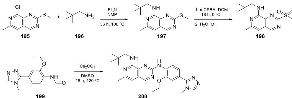
Scheme 20. N8-(2,2-dimethylpropyl)-N2-[2-ethoxy-4-(4-methyl-4H-1,2,4-triazol-3-yl)phenyl]-6-methylpyrido[3,4-d]pyrimidine-2,8-diamine ( 200 ), BOS172722 [62].
