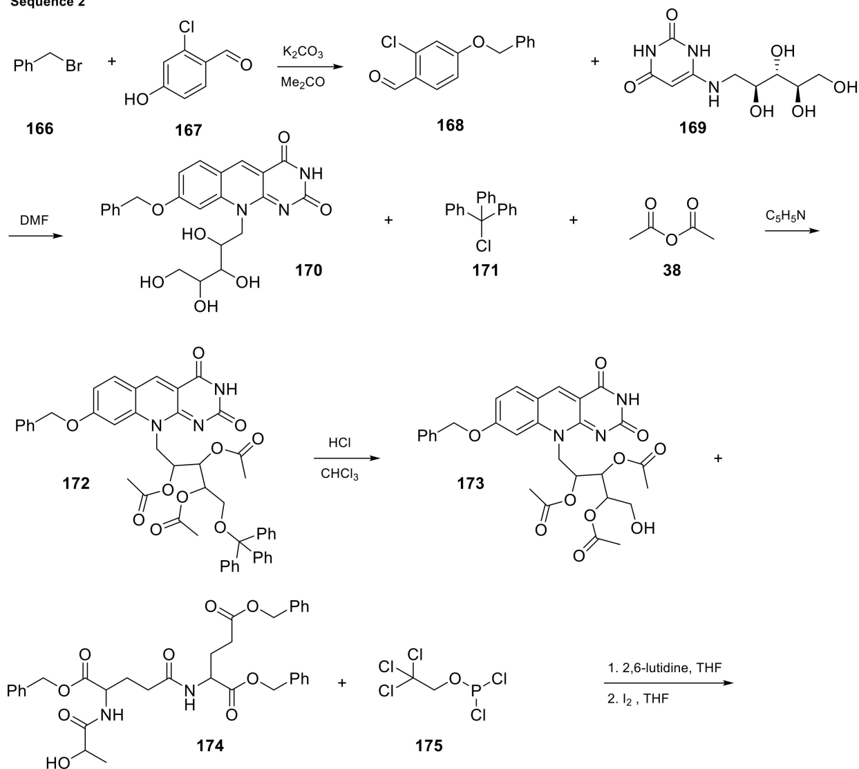
Scheme 18. Cont.
