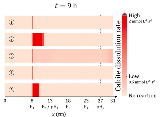
Fig. 9. Reactive zone location for the different experiments of calcite dissolution from the dissolution rate extracted from the numerical simulations at 9 h after the start of acid injection for the five experiments. The same color scale is used for all of the experiments. The maximum value is set to 2 \text{ mmol L}^{-1} \text{ s}^{-1} , but the red color indicates values that can be higher.
