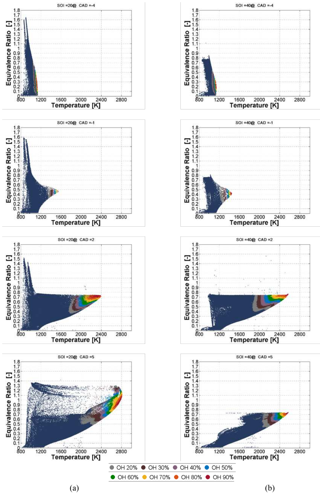
Figure 35. In-cylinder equivalence ratio and temperature distributions from CFD calculations corresponding to different CAD for SOI = -20 CAD (a) and SOI = -40 CAD (b). Relative Iso-contours of OH normalized concentrations are also reported. Initial conditions are reported in Table 5 .
